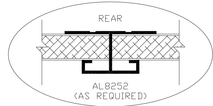
TOP SECTION VIEW SCALE: 1/2
