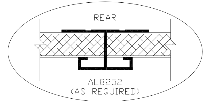
TOP SECTION VIEW SCALE: 1/2
