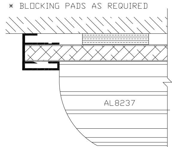
TOP SECTION VIEW SCALE: 1/2
