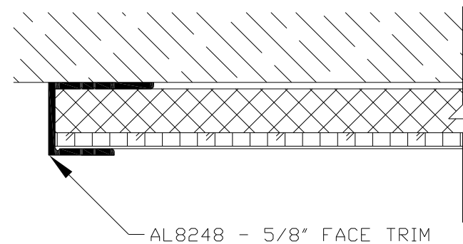
TOP SECTION
